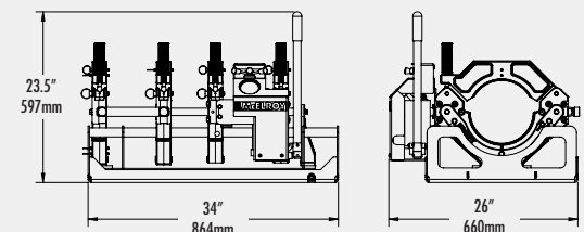
DYNAMC 28 HP 4-JAW
