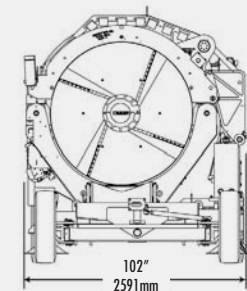
MEGAMC 1600
