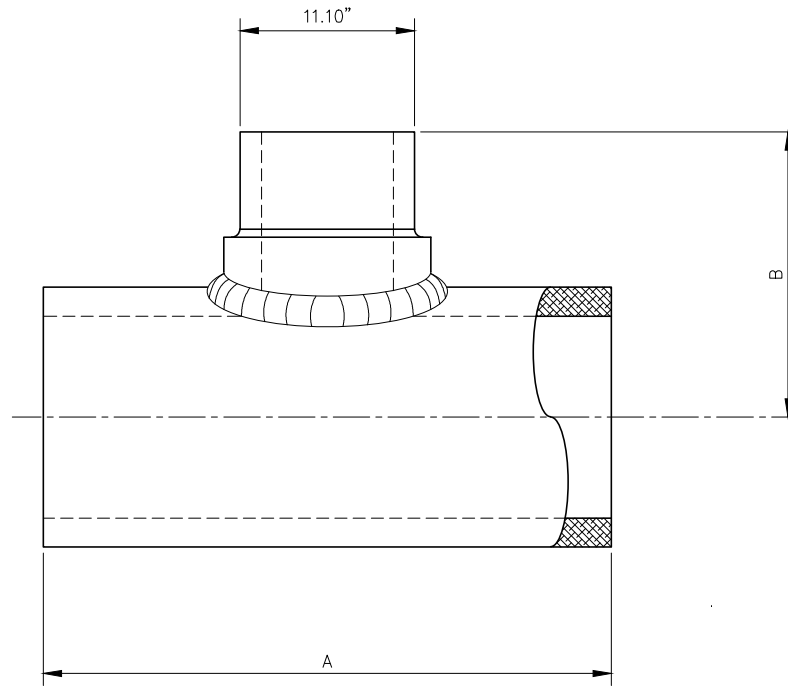
10" OUTLET BRANCH SADDLE TEE SCALE: NTS
