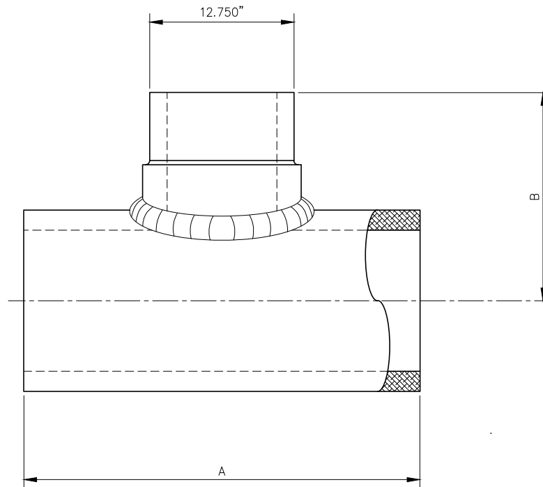
12" OUTLET BRANCH SADDLE TEE SCALE: 1"=1'-0"
