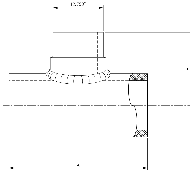
12" OUTLET BRANCH SADDLE TEE SCALE: NTS
