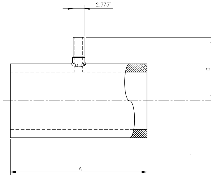
2" OUTLET BRANCH SADDLE TEE SCALE: NTS
