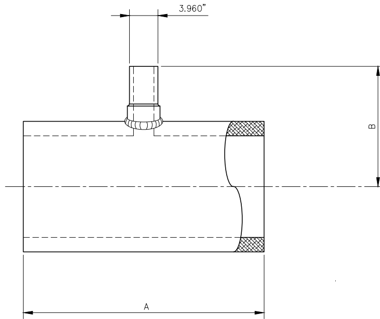
3" OUTLET BRANCH SADDLE TEE SCALE: NTS
