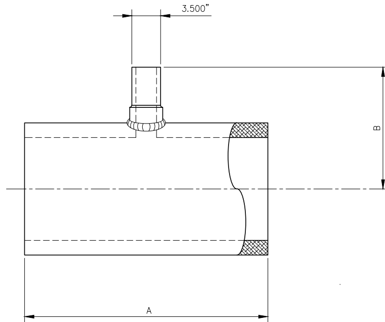
3" OUTLET BRANCH SADDLE TEE SCALE: NTS
