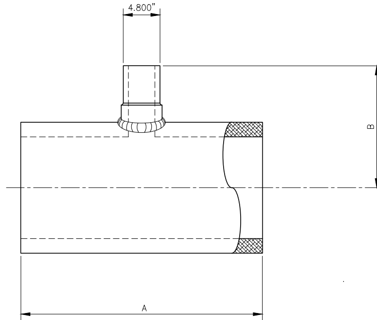
4" OUTLET BRANCH SADDLE TEE SCALE: NTS
