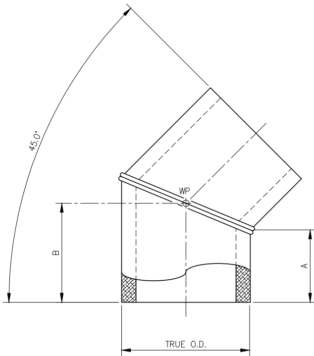
45° ELBOW, 2-SEGMENT SCALE: NTS
