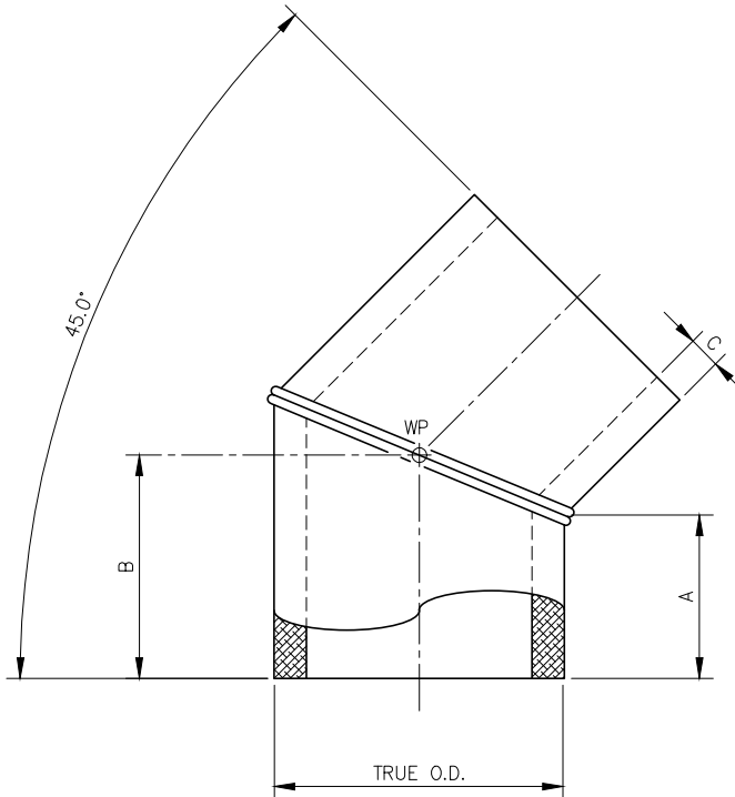
45° ELBOW, 2-SEGMENT SCALE: NTS
