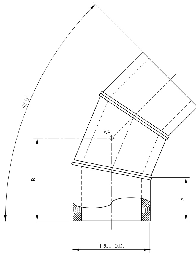
45° ELBOW, 3-SEGMENT SCALE: NTS
