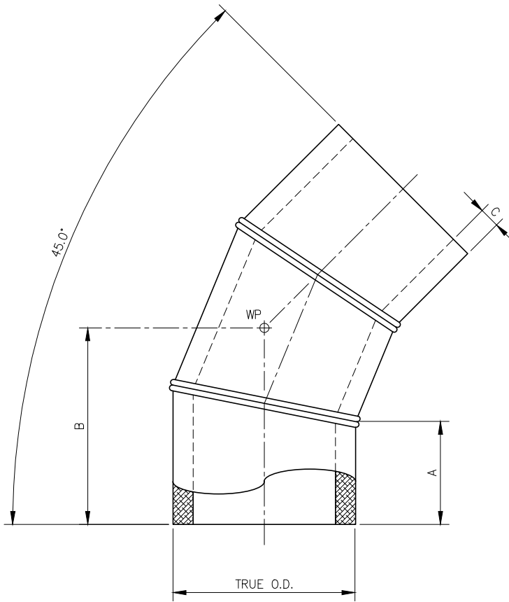
45° ELBOW, 3-SEGMENT SCALE: NTS
