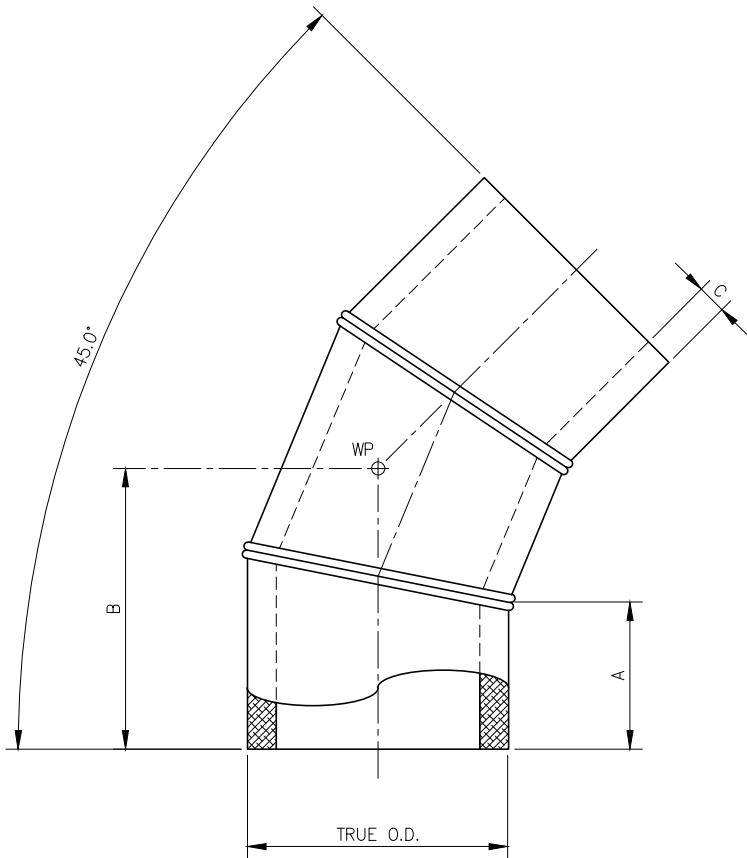
45° ELBOW, 3-SEGMENT SCALE: NTS
