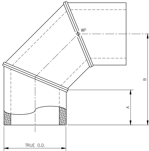
90° ELBOW, 3-SEGMENT SCALE: NTS
