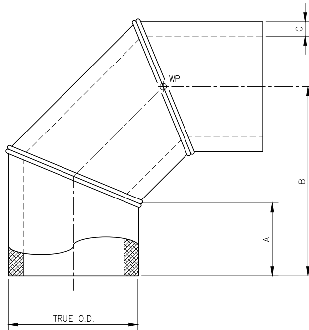
90° ELBOW, 3-SEGMENT SCALE: NTS
