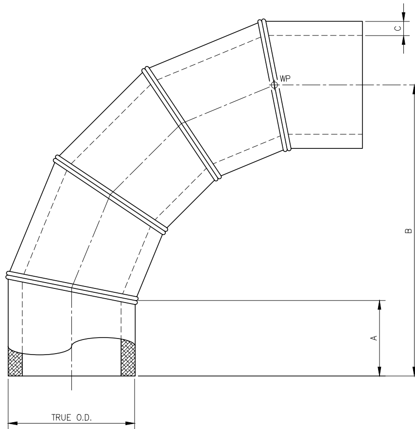
90° ELBOW, 5-SEGMENT
