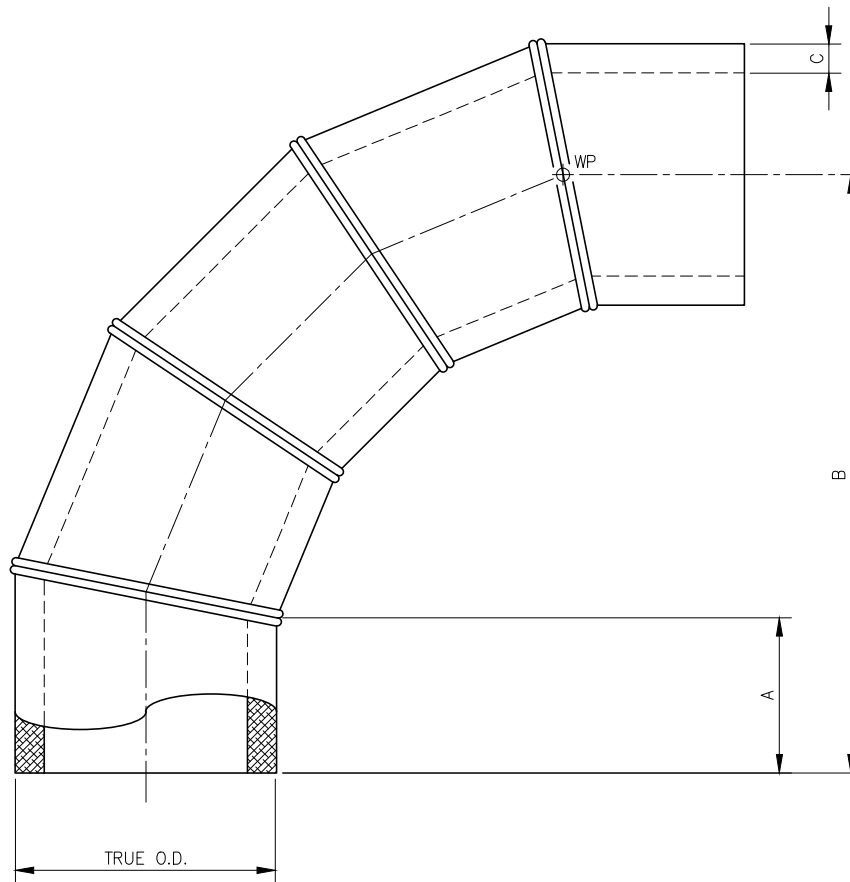
90° ELBOW, 5-SEGMENT
