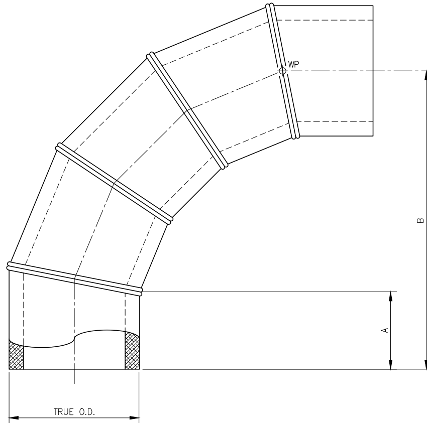
90° ELBOW, 5-SEGMENT
