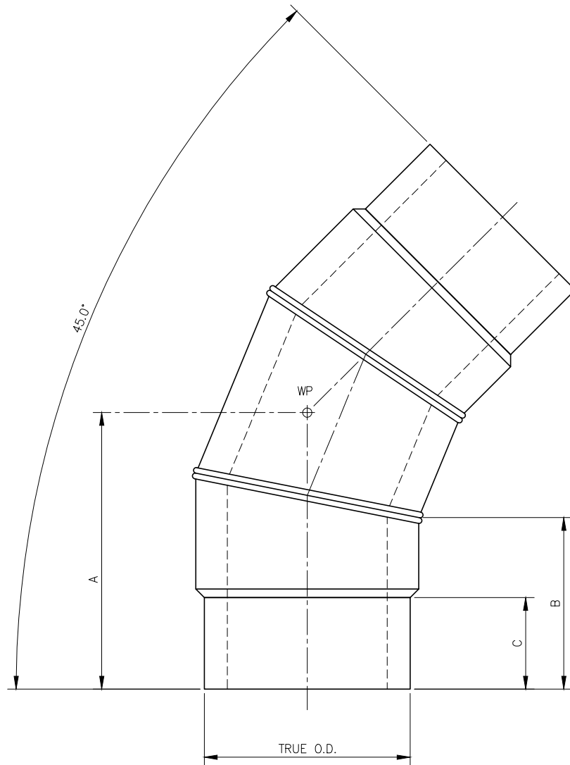
45° ELBOW, 3-SEGMENT SCALE: 1"=1'-0"
