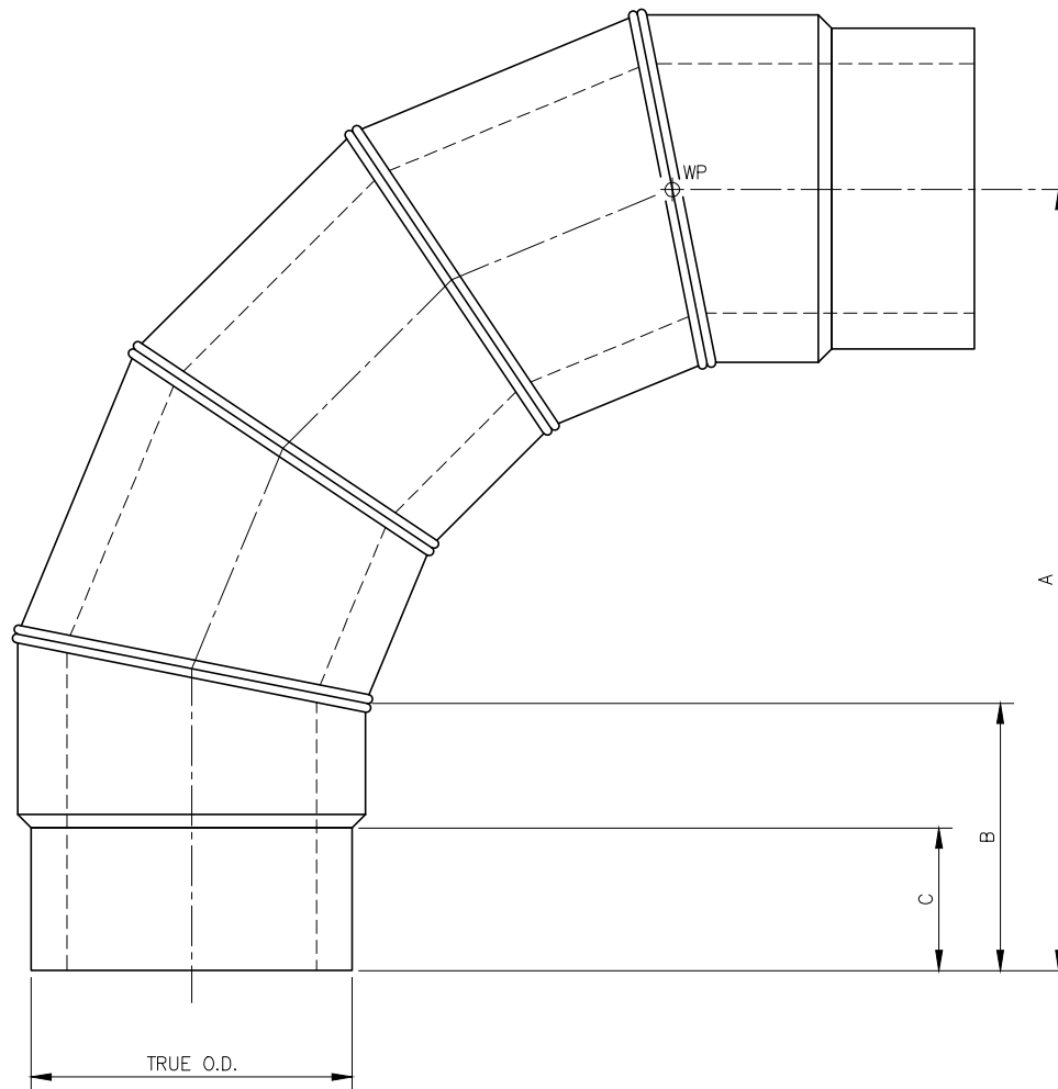
90° ELBOW, 5-SEGMENT SCALE: 1"=1'-0"
