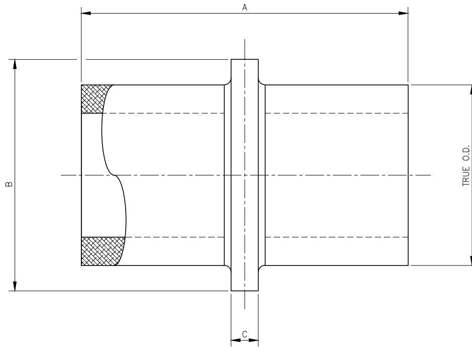
WATER-STOP SCALE: NTS
